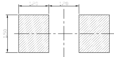
推荐焊盘尺寸 Recommended Soldering Pad
