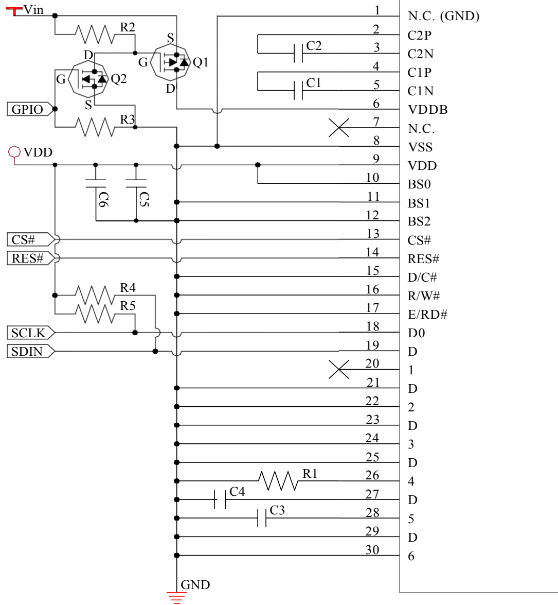
3-wire serial interface
