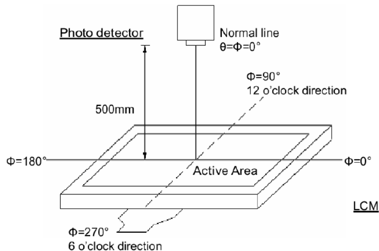
Fig. 4-2 Optical measurement system setup
