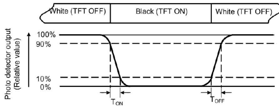
Fig. 4-3 Definition of response time
