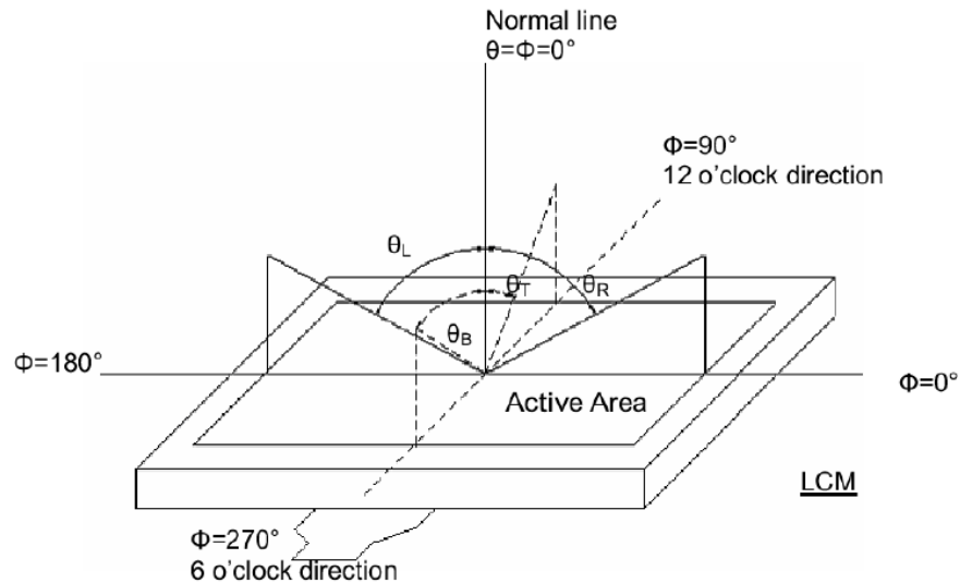
Fig. 4-1 Definition of viewing angle
