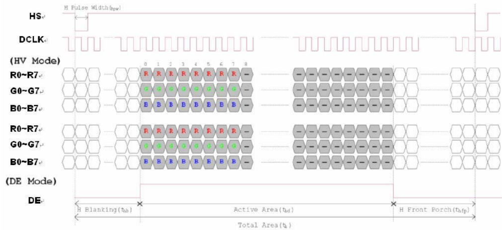
Figure 3. 1 Horizontal input timing diagram.
