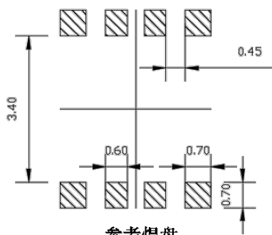
参考焊盘 Reference Soldering Pad
