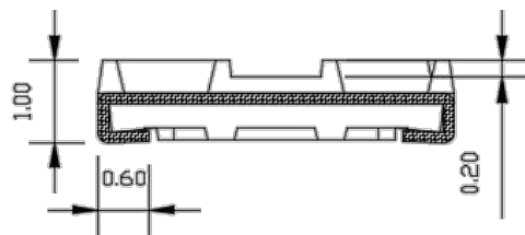
剖面图 Cutaway view
