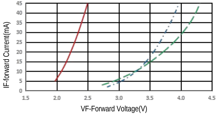
Electrical Characteristics
