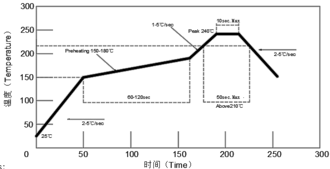
Recommended Reflow Soldering Curve
