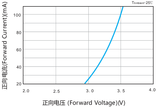
Volt-Ampere Characteristics
