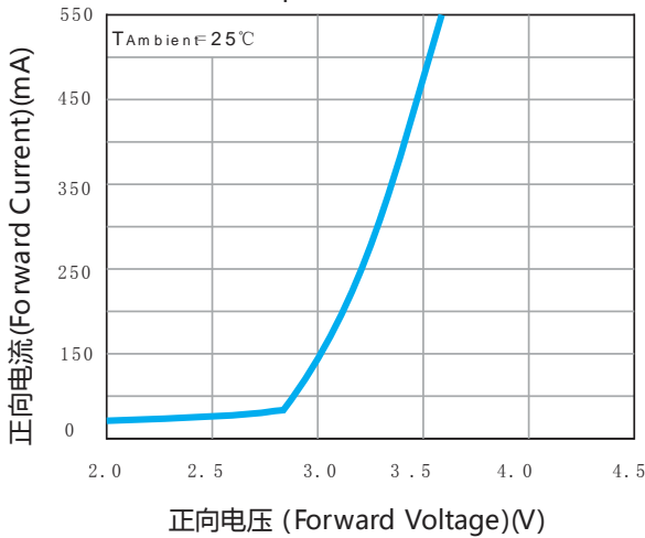
Volt-Ampere Characteristics
