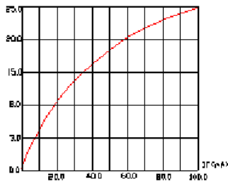
FIG.3 RELATIVE LUMINOUS INTENSITY VS FORWARD CURRENT
