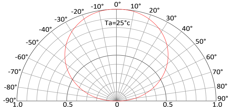
Radiation Pattern
