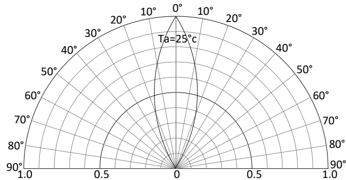
Radiation Pattern
