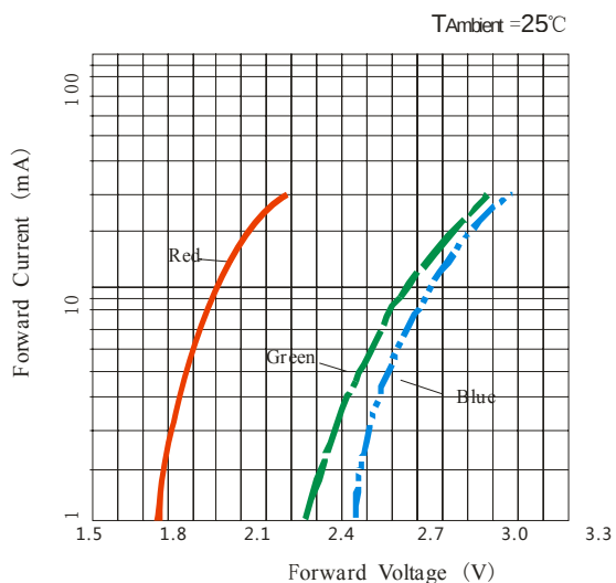
Volt-Ampere Characteristics
