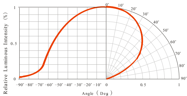
Typical Spatial Distribution
