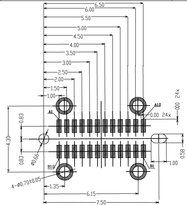
RECOMMENDED P.C.B. LAYOUT (T:1.00mm) TOLERANCE UNSPECIFIED ±0.05mm SCALE 2:1
