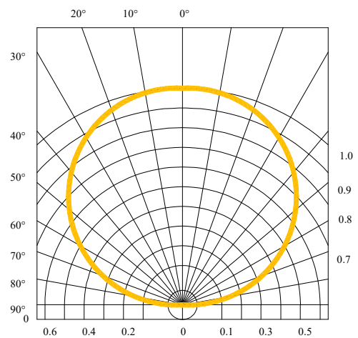
Radiation Diagram
