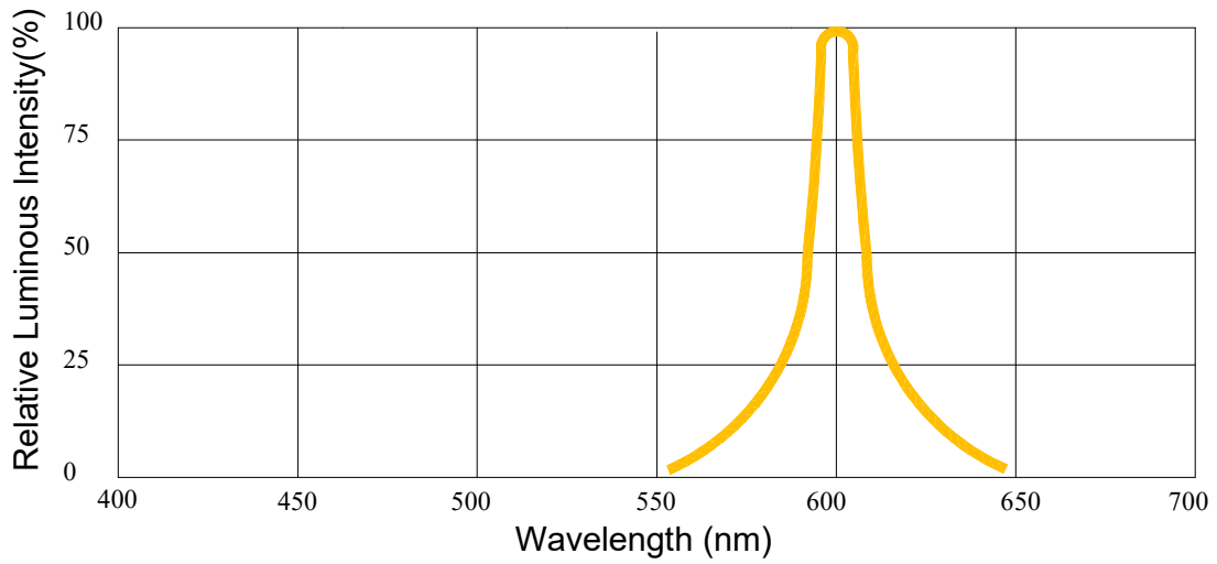
Spectrum Distribution
