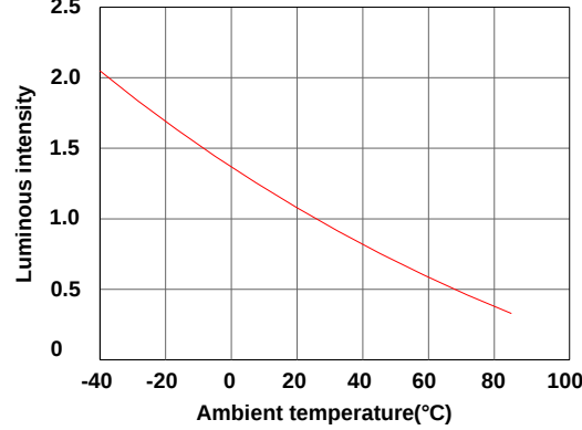
Luminous Intensity vs.Ambient Temperaturs
