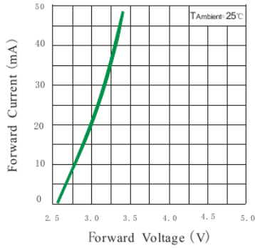
Volt-Ampere Characteristics
