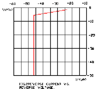
FIG.2 REVERSE CURRENT VS REVERSE VOLTAGE
