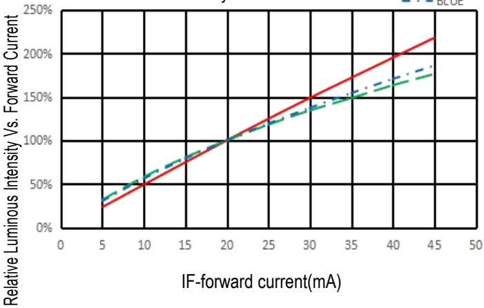
Relative Luminous Intensity Vs. Forward Current
