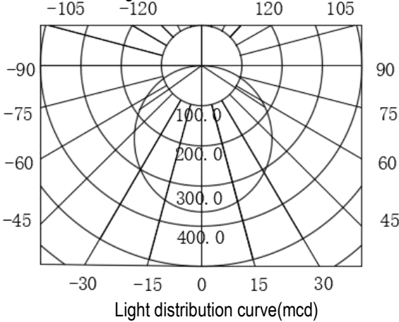
Light Distribution Curve
