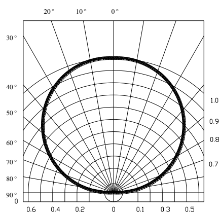
Radiation Diagram
