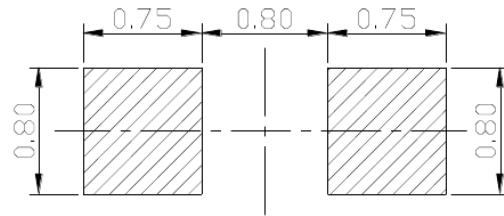
推荐焊盘尺寸 Recommended Soldering Pad
