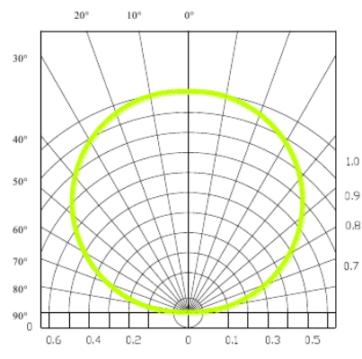
Radiation Diagram
