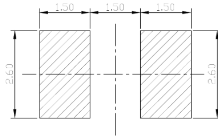
推荐焊盘 Recommended Soldering Pad
