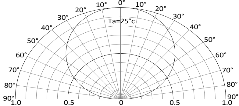
Radiation Pattern
