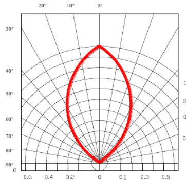
Radiation Diagram
