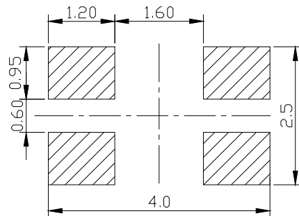
推荐焊盘 Recommended Soldering Pad
