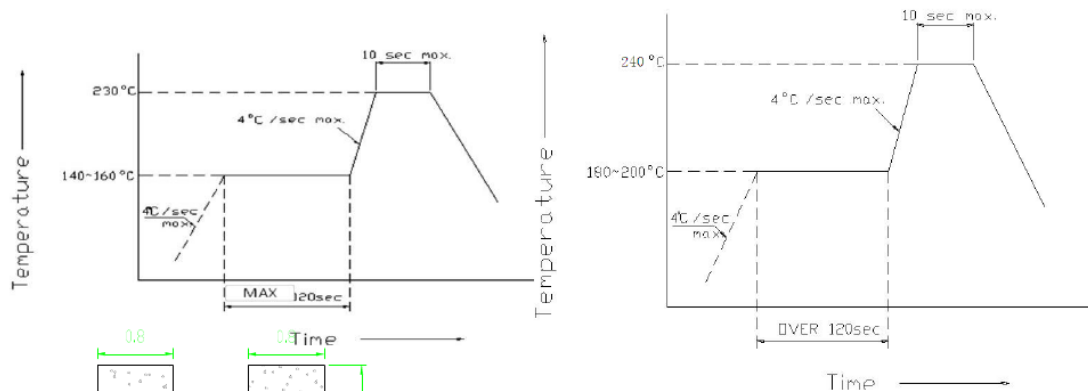
Recommended Soldering Pattern (Units : mm)
