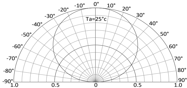
Radiation Pattern
