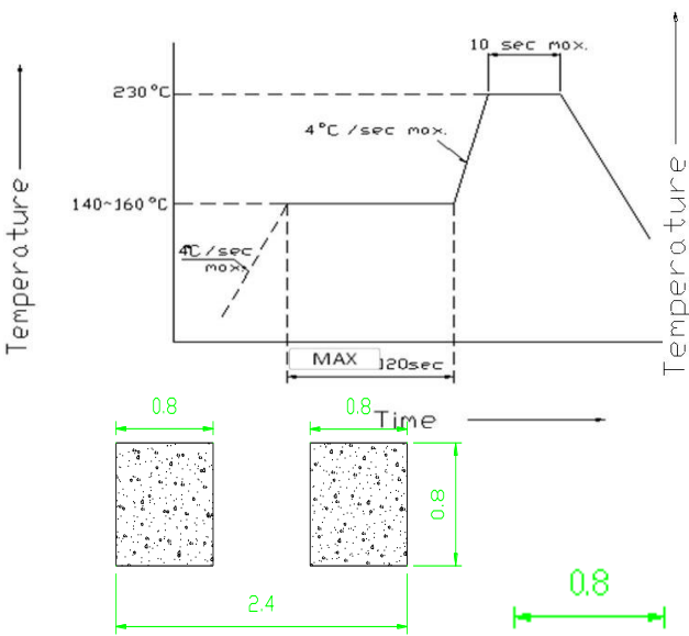
Recommended Soldering Pattern (Units : mm)
