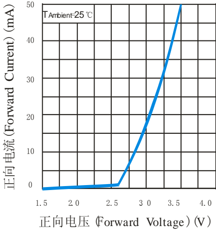
Volt-Ampere Characteristics
