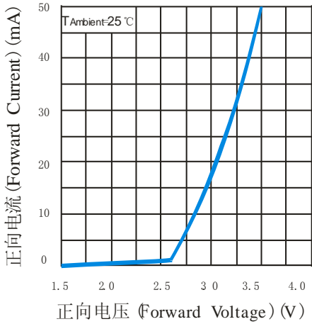
Volt-Ampere Characteristics
