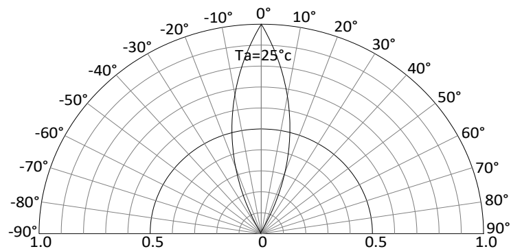
Radiation Pattern
