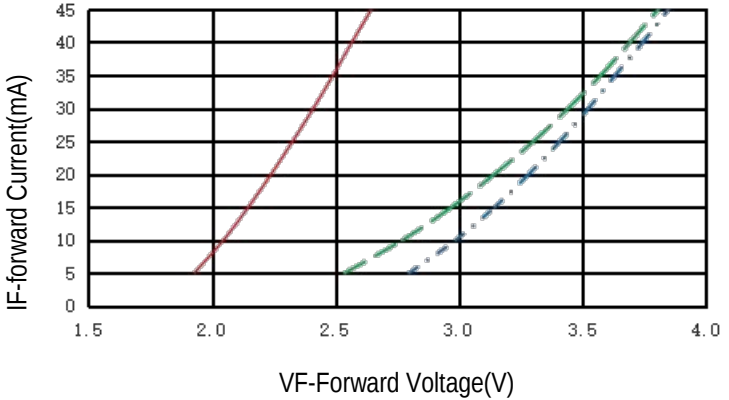
Electrical Characteristics
