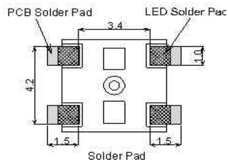
Solder Pad
