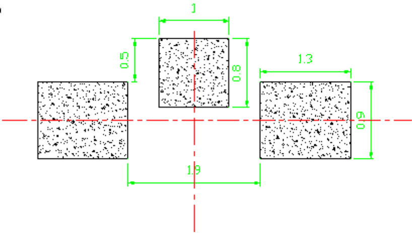
Recommended Solder Pad Dimensions (Units : mm)
