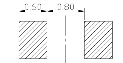
Recommended Soldering Pad
