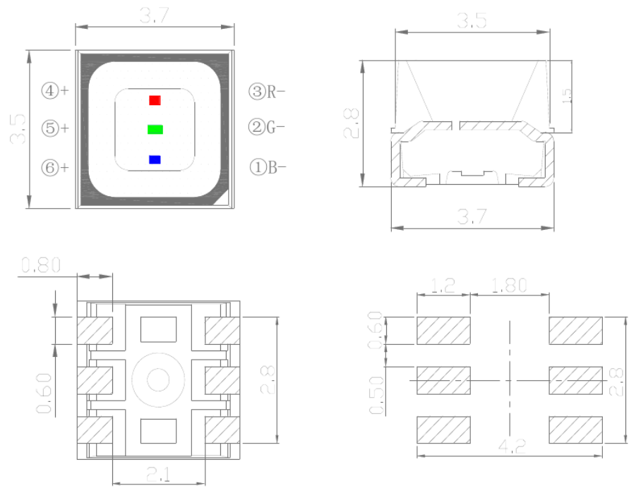
推荐焊盘 Recommended Soldering Pad
