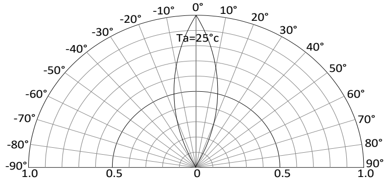
Radiation Pattern
