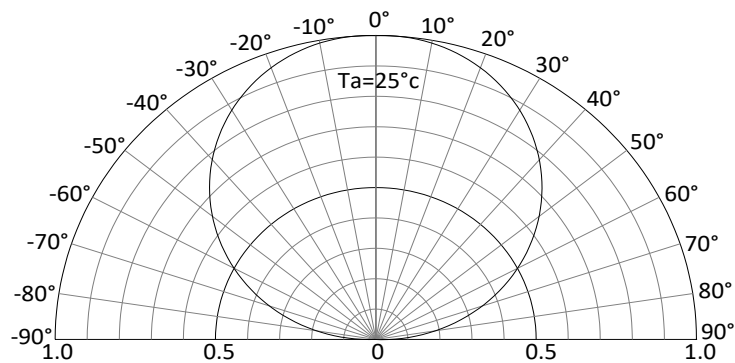
Radiation Pattern
