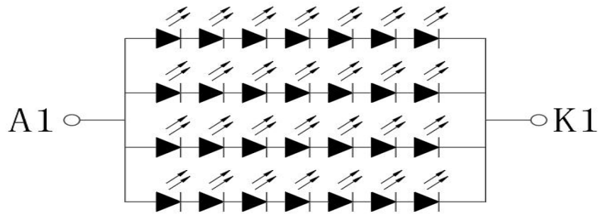
LED CIRCUIT DIAGRAM
