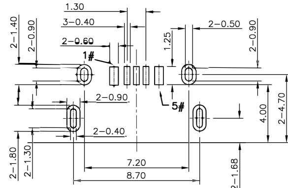
RECOMMENDED P.C.B. LAYOUT (TOP VIEW) GENERAL TOLERANCE: \pm 0.05
